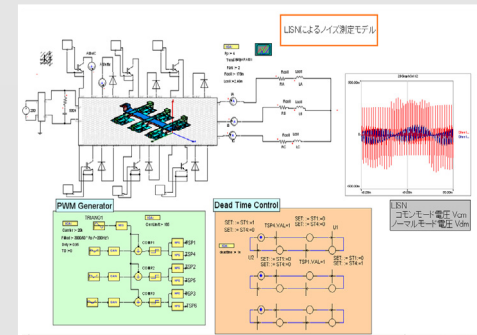
Simplorer can simulate complete systems including inverter, control algorithms and rigid body dynamics
